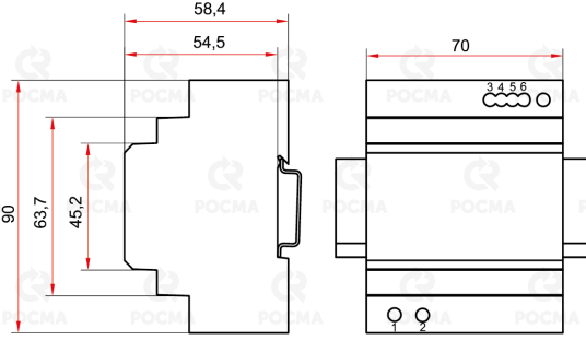
HDR-100-24
